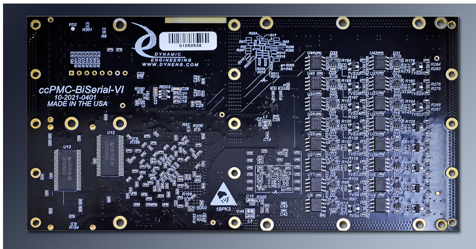
Figure 1 ccPMC-BiSerial-VI-GPIO REAR VIEW
